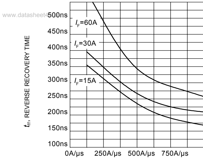
Figure 21. Typical reverse recovery time as a function of diode current slope ( V_R=400V , T_J=150^\circ C , Dynamic test circuit in Figure E)
